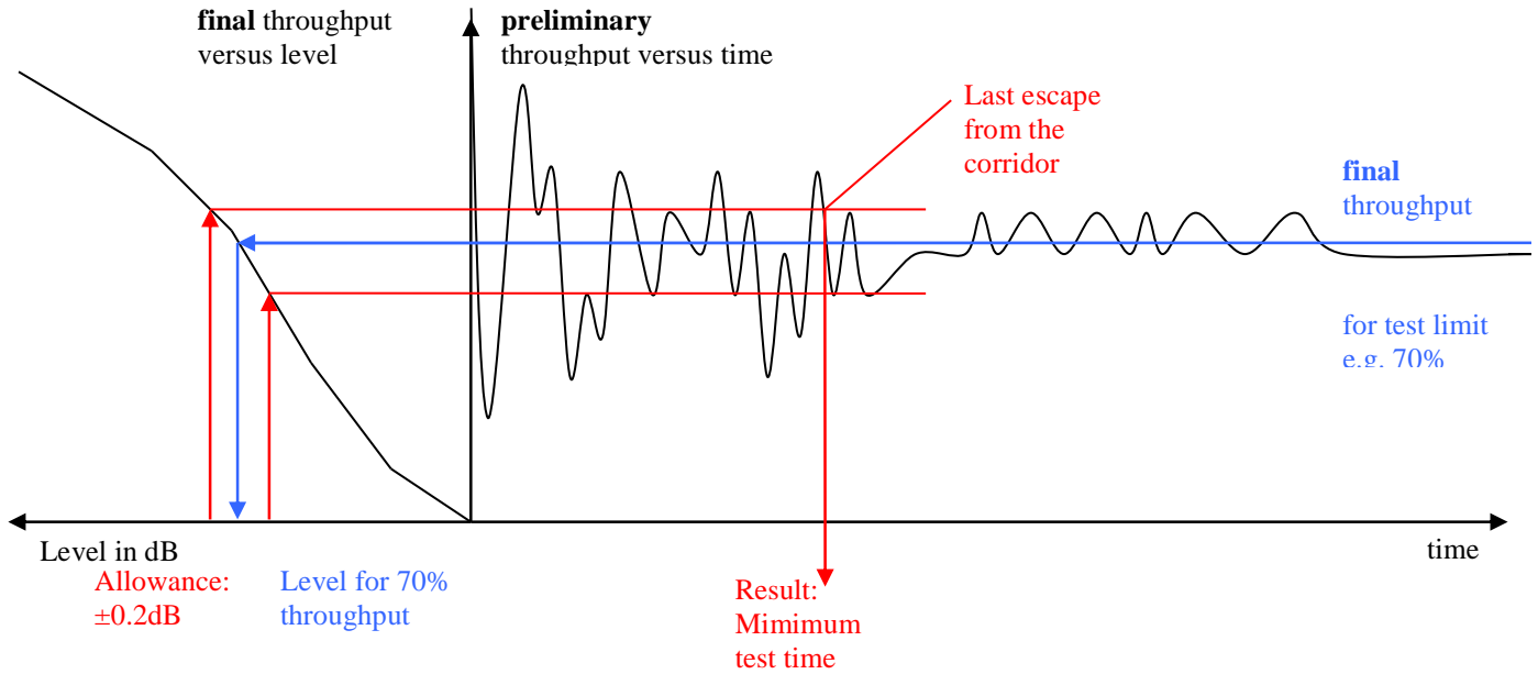
Figure G.1.5-1: Simulation method to derive minimum test time
