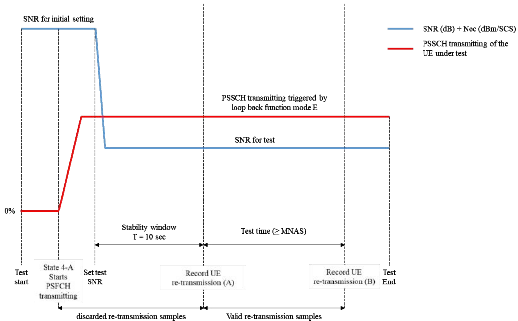
Figure G.5.3-1: Proposed Test Method for PSFCH performance
