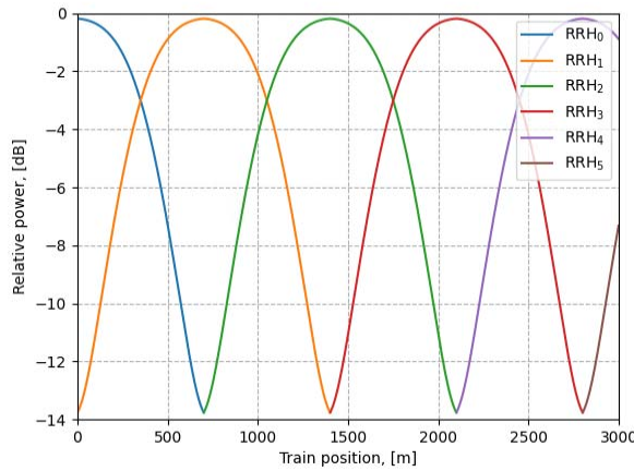
Figure B.3.6-2: Relative power level trajectories
