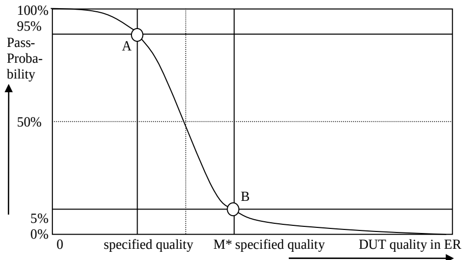
Figure G.2.8-1: Pass probability versus DUT quality
