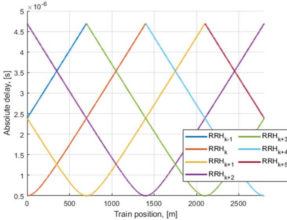
Figure B.3.2-5 Absolute delay trajectories
