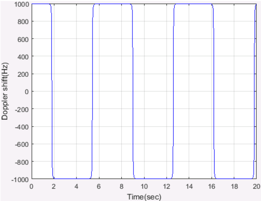
Figure B.3.1-2: Doppler shift trajectory ( f_d = 1000 Hz)
