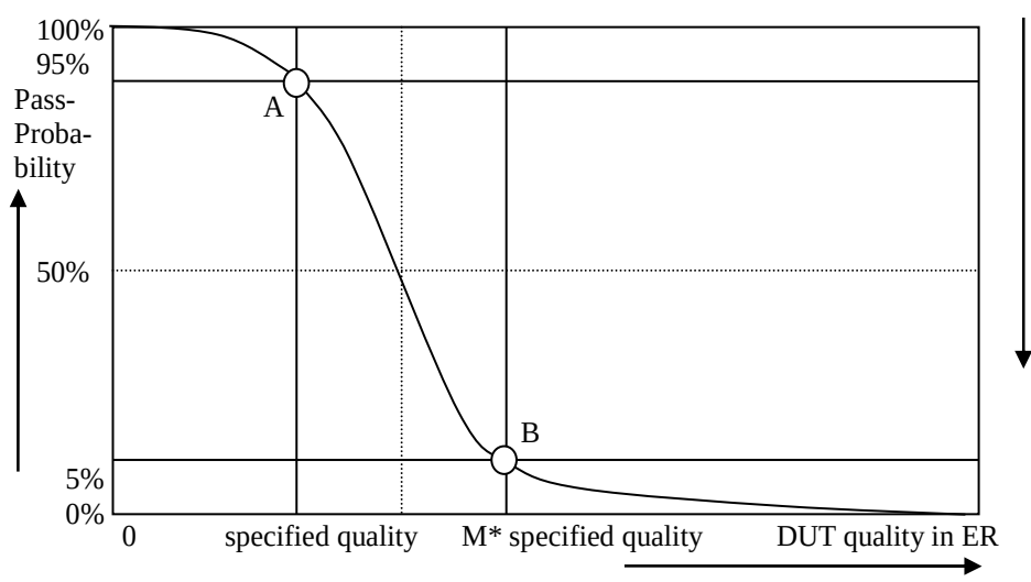
Figure G.2.8-1: Pass probability versus DUT quality
