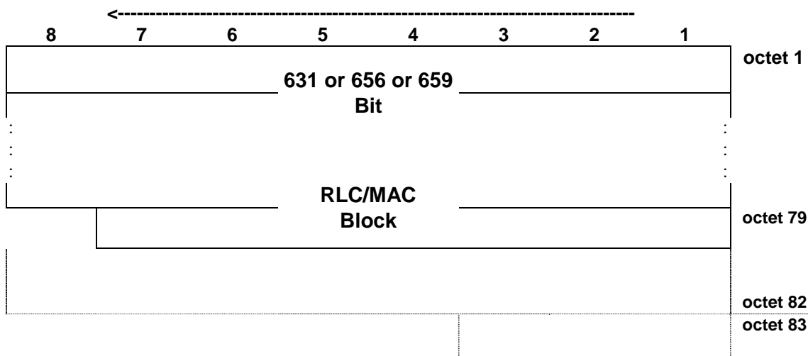
Figure 7.6.10.1: PDTCH block type 10 (MCS-6) uplink format
