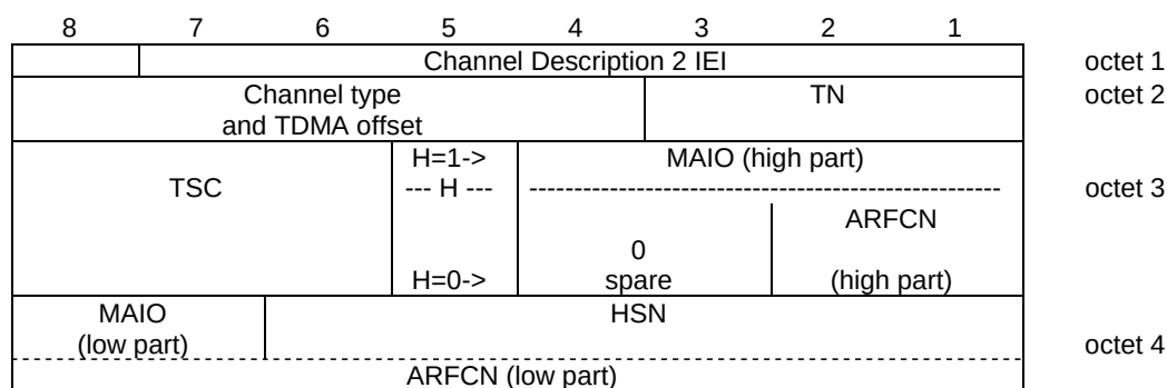
Figure 10.5.2.5a.1: Channel Description 2 information element
