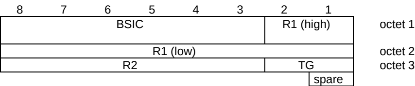
Figure 9.1.30b.1: COMPACT Frame synchronization information element
