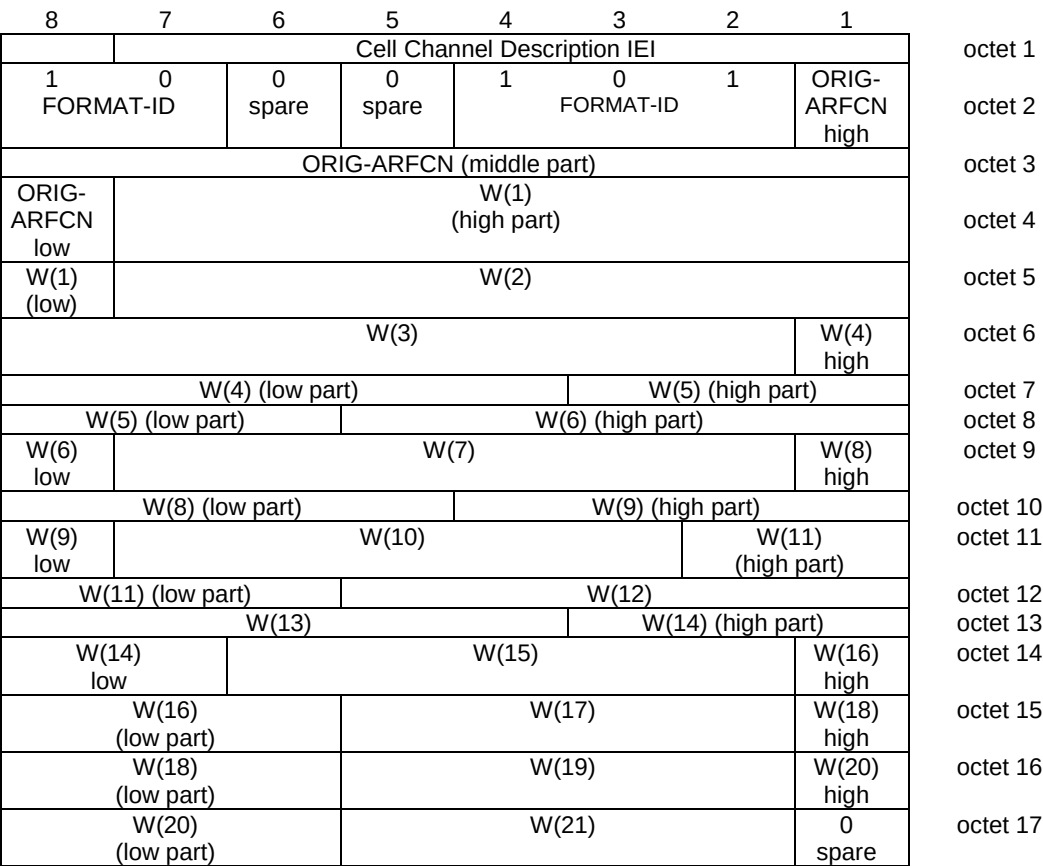
Figure 10.5.2.1b.5.1: Cell Channel Description information element, range 256 format
