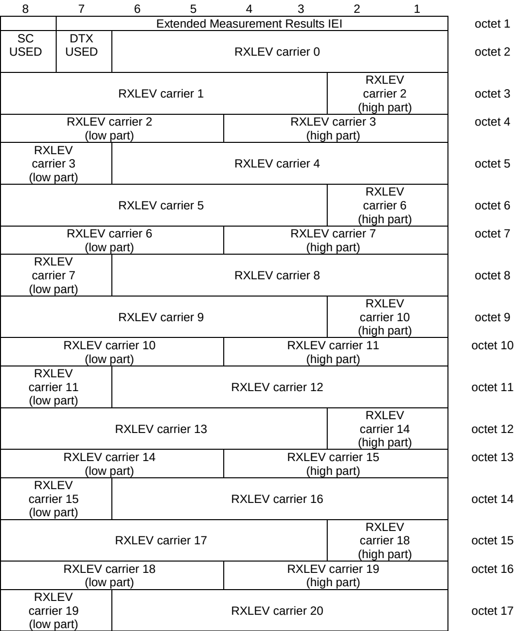
Figure 10.5.2.45.1: Extended Measurement Results information element
