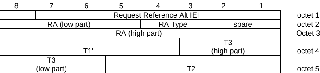
Figure 10.5.2.87.1: Request Reference Alt information element
