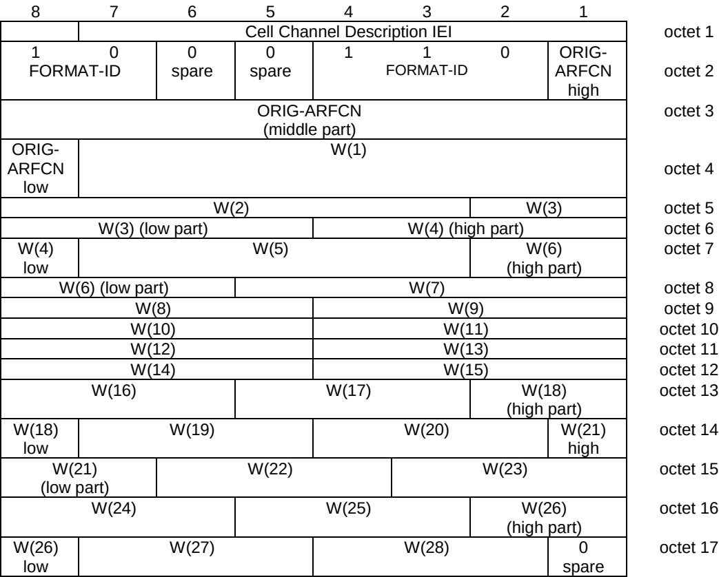
Figure 10.5.2.1b.6.1: Cell Channel Description information element, range 128 format
