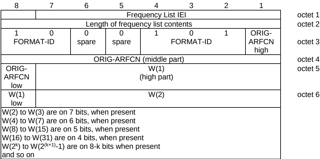
Figure 10.5.2.13.5.1: Frequency List information element (Range 256 format)
