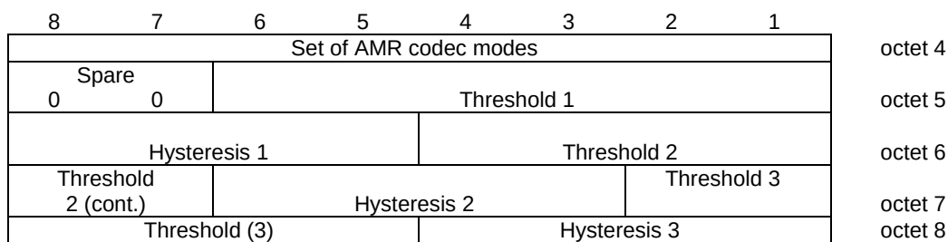
Figure 10.5.2.21aa.5: Parameters for multirate speech field for the Multirate speech versions 1 & 2 when a set of four modes is chosen
