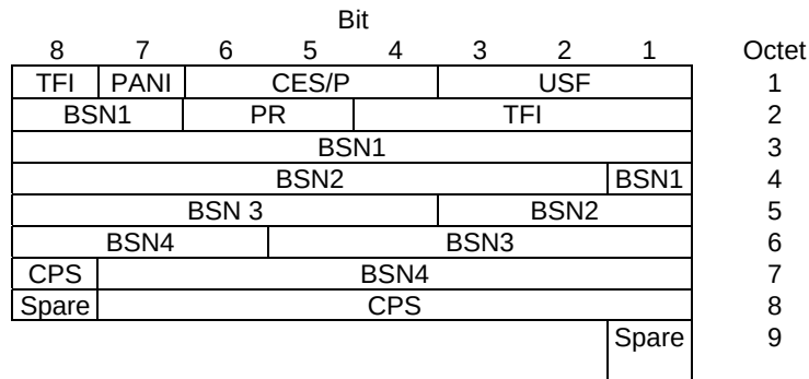
Figure 10.3a.3.9.1: Combined downlink RLC data block header for DBS-11 and DBS-12.
