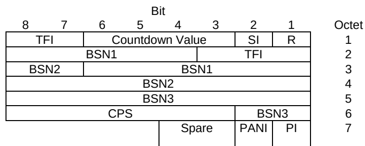
Figure 10.3a.4.5.1: Combined uplink RLC data block header for UAS-10, UAS-11.
