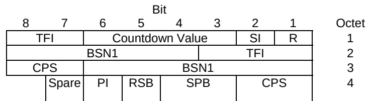
Figure 10.3a.4.3.1: EGPRS uplink RLC data block header (FANR not activated) for MCS-1, MCS-2, MCS-3 and MCS-4
