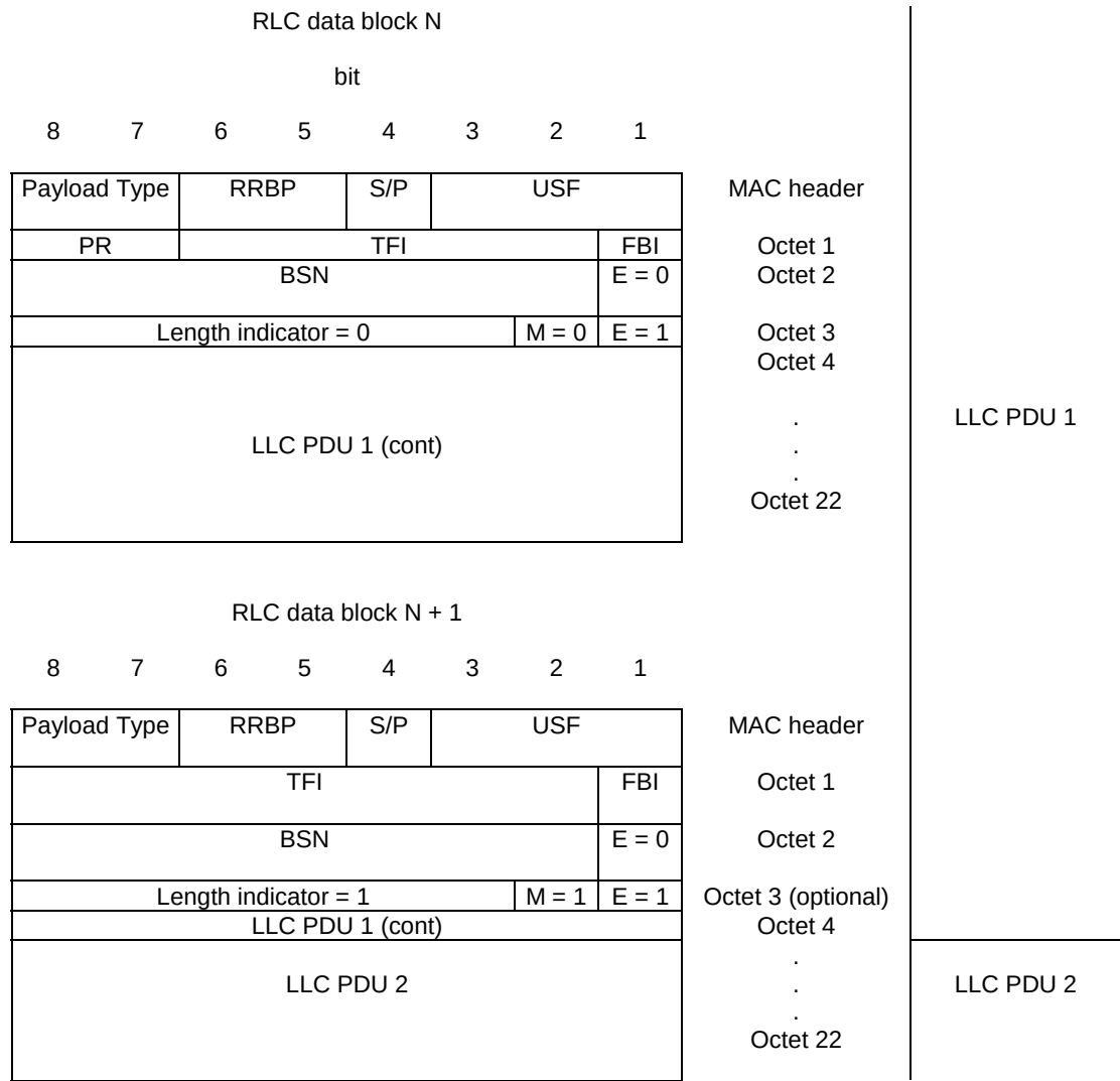
Figure B.2: Length indicator (LI) example
