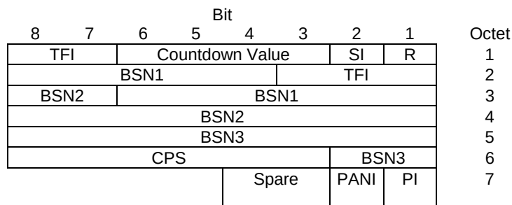
Figure 10.3a.4.8.1: Combined uplink RLC data block header for UBS-9, UBS-10.
