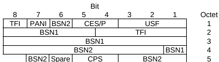
Figure 10.3a.3.10.2: DLMC Combined downlink RLC data block header for DAS-10.
