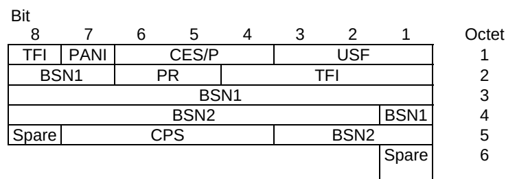
Figure 10.3a.3.7.1: Combined downlink RLC data block header for DBS-7 and DBS-8.
