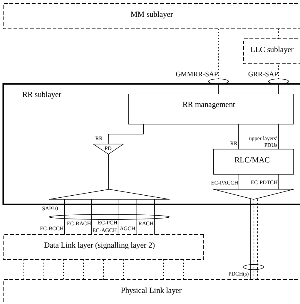
Figure 4.2: Protocol architecture of Radio Resource (RR) sublayer and RLC/MAC function in EC operation
