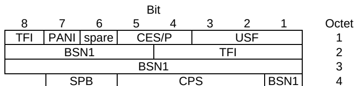
Figure 10.3a.3.3.5: DLMC EGPRS (FANR activated) / DLMC EGPRS2 downlink RLC data block header for MCS-1, MCS-2, MCS-3 and MCS-4
