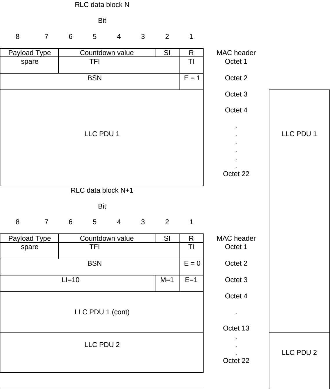
Figure B.7: Example when Length indicator (LI) can be omitted
