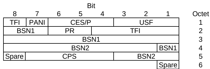
Figure 10.3a.3.4.1: Combined downlink RLC data block header for DAS-8 and DAS-9.
