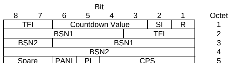
Figure 10.3a.4.7.1: Combined uplink RLC data block header for UBS-7, UBS-8.
