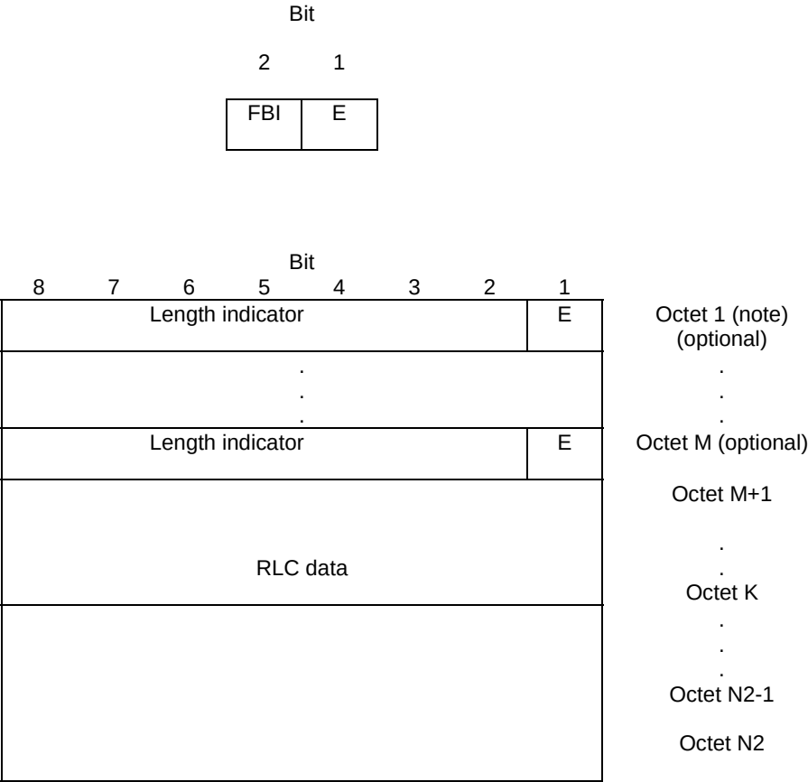
Figure 10.3a.1.2.1: EC-GSM-IoT downlink RLC data block
