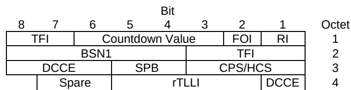
Figure 10.3a.4.3.3: EC-GSM-IoT uplink RLC data block header for MCS-1, MCS-2, MCS-3 and MCS-4
