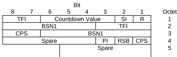
Figure 10.3a.4.2.1: EGPRS uplink RLC data block header (FANR not activated) for MCS-5 and MCS-6
