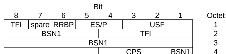
Figure 10.3a.3.2.3: DLMC EGPRS downlink RLC data block header (FANR not activated) for MCS-5 and MCS-6
