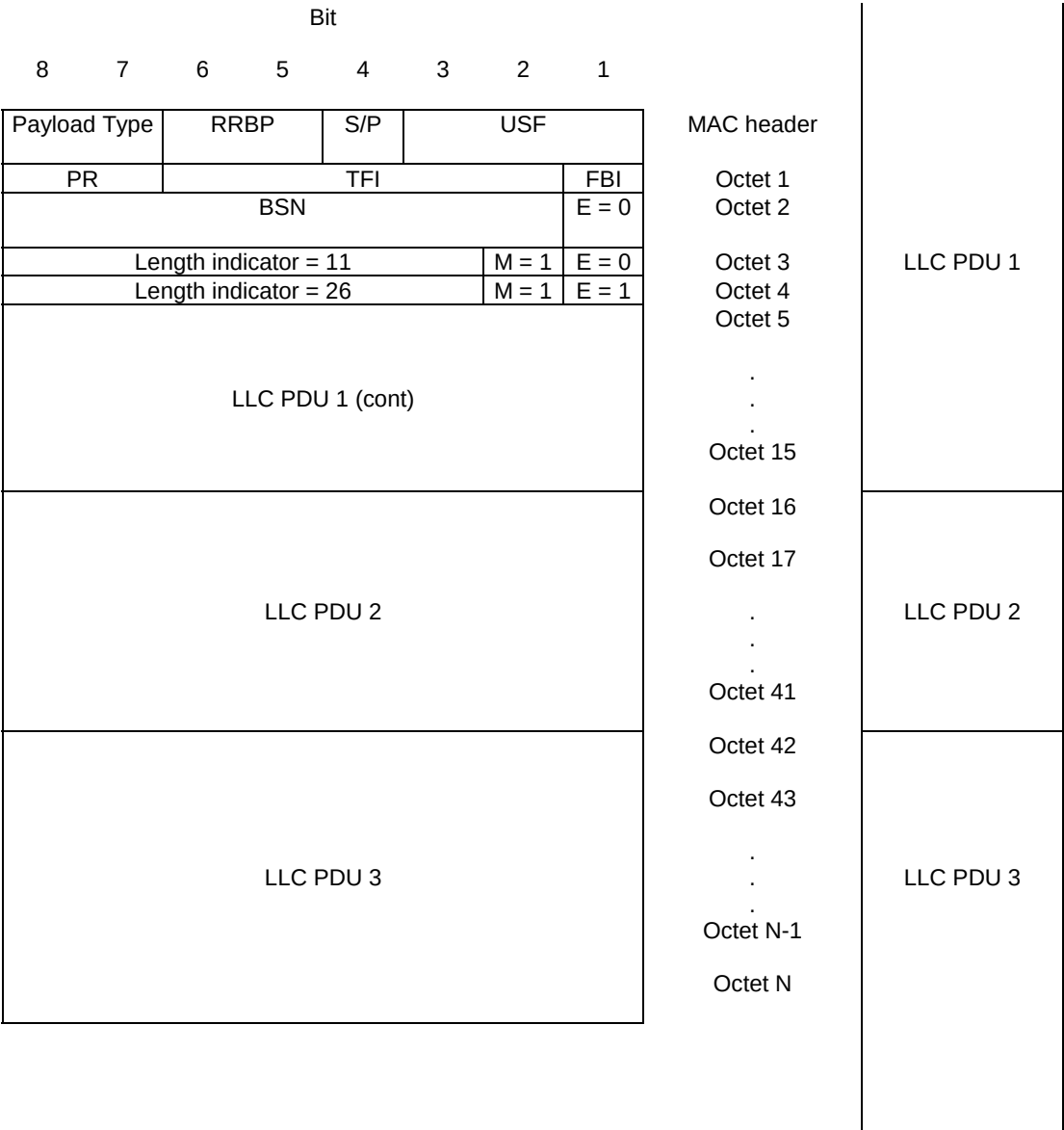
Figure B.1: Length indicator (LI) example
