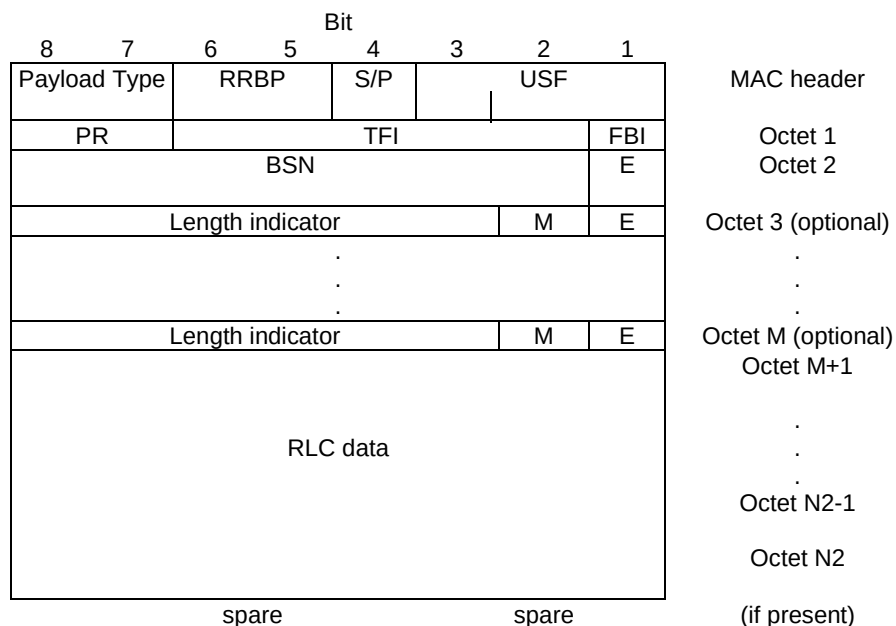
Figure 10.2.1.1: Downlink RLC data block with MAC header
