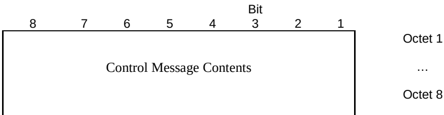
Figure 10.3.2.2: EC-GSM-IoT Uplink RLC/MAC control block.
