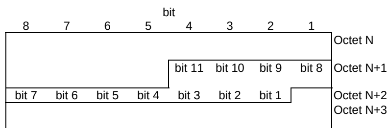
Figure 11.1: Field mapping within RLC/MAC messages
