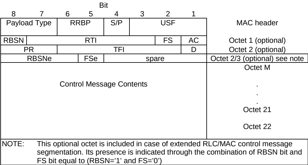
Figure 10.3.1.1.1: Downlink RLC/MAC control block together with its MAC header
