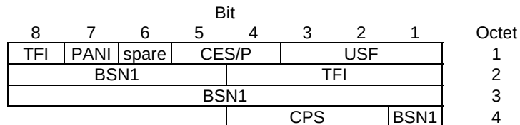
Figure 10.3a.3.2.4: DLMC EGPRS (FANR activated) / DLMC EGPRS2 downlink RLC data block header for MCS-5, MCS-6, DAS-5, DAS-6 and DAS-7
