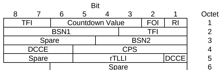
Figure 10.3a.4.1.3: EC-GSM-IoT uplink RLC data block header for MCS-7, MCS-8 and MCS-9.
