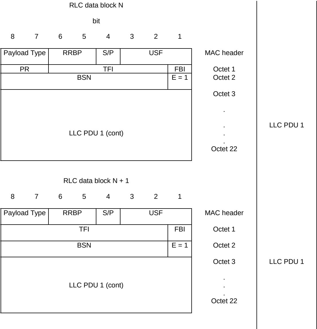
Figure B.4: Example when Length indicator (LI) can be omitted
