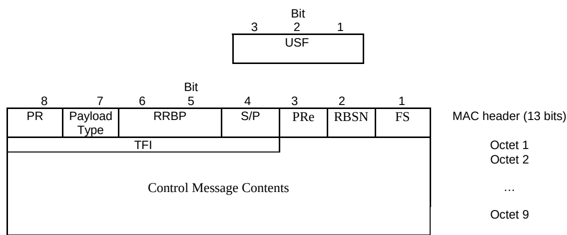
Figure 10.3.1.3.2: EC-GSM-IoT Downlink RLC/MAC control block together with its extended MAC header when Payload Type is set to 1
