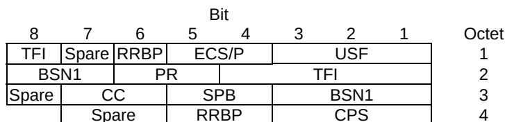
Figure 10.3a.3.3.6: EC-GSM-IoT downlink RLC data block header for MCS-1, MCS-2, MCS-3 and MCS-4
