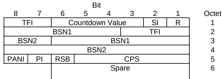
Figure 10.3a.4.1.2: EGPRS uplink RLC data block header (FANR activated) for MCS-7, MCS-8 and MCS-9.
