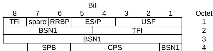
Figure 10.3a.3.3.4: DLMC EGPRS downlink RLC data block header (FANR not activated) for MCS-1, MCS-2, MCS-3 and MCS-4
