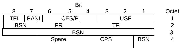
Figure 10.3a.3.6.1: Combined downlink RLC data block header for DBS-5 and DBS-6.
