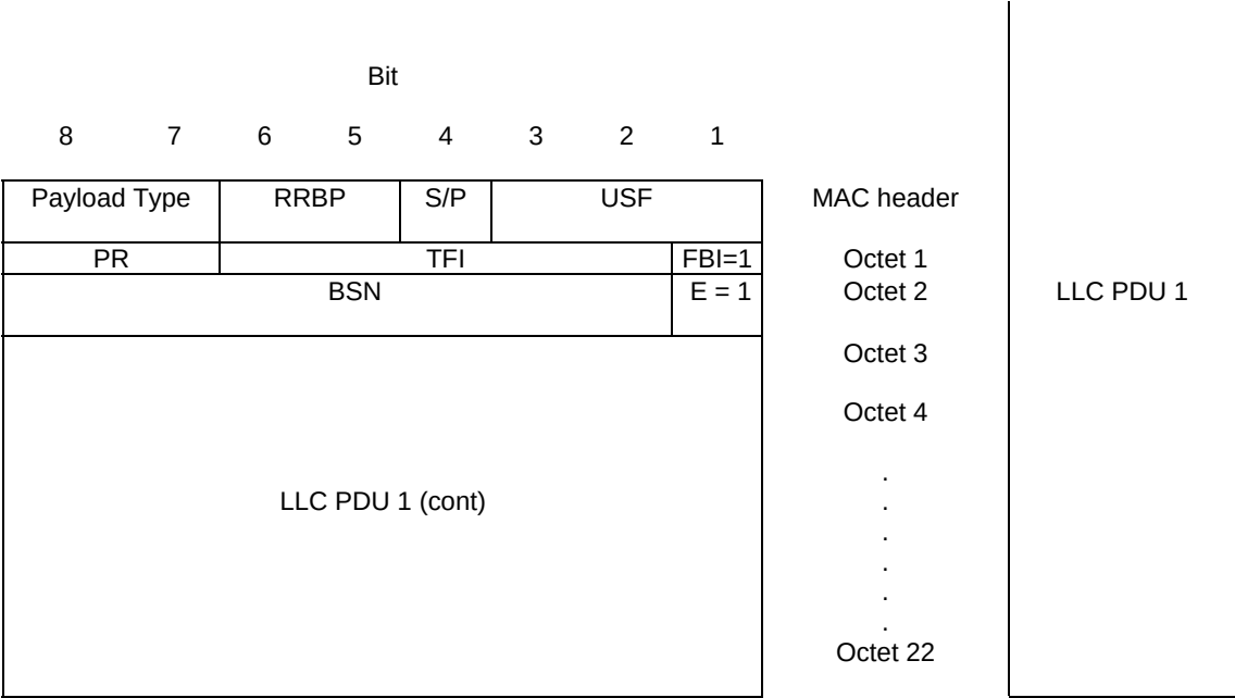
Figure B.5: Example when Length indicator (LI) can be omitted
