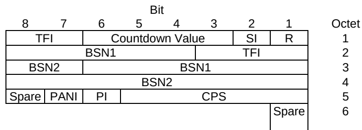
Figure 10.3a.4.4.1: Combined uplink RLC data block header for UAS-7, UAS-8 and UAS-9.
