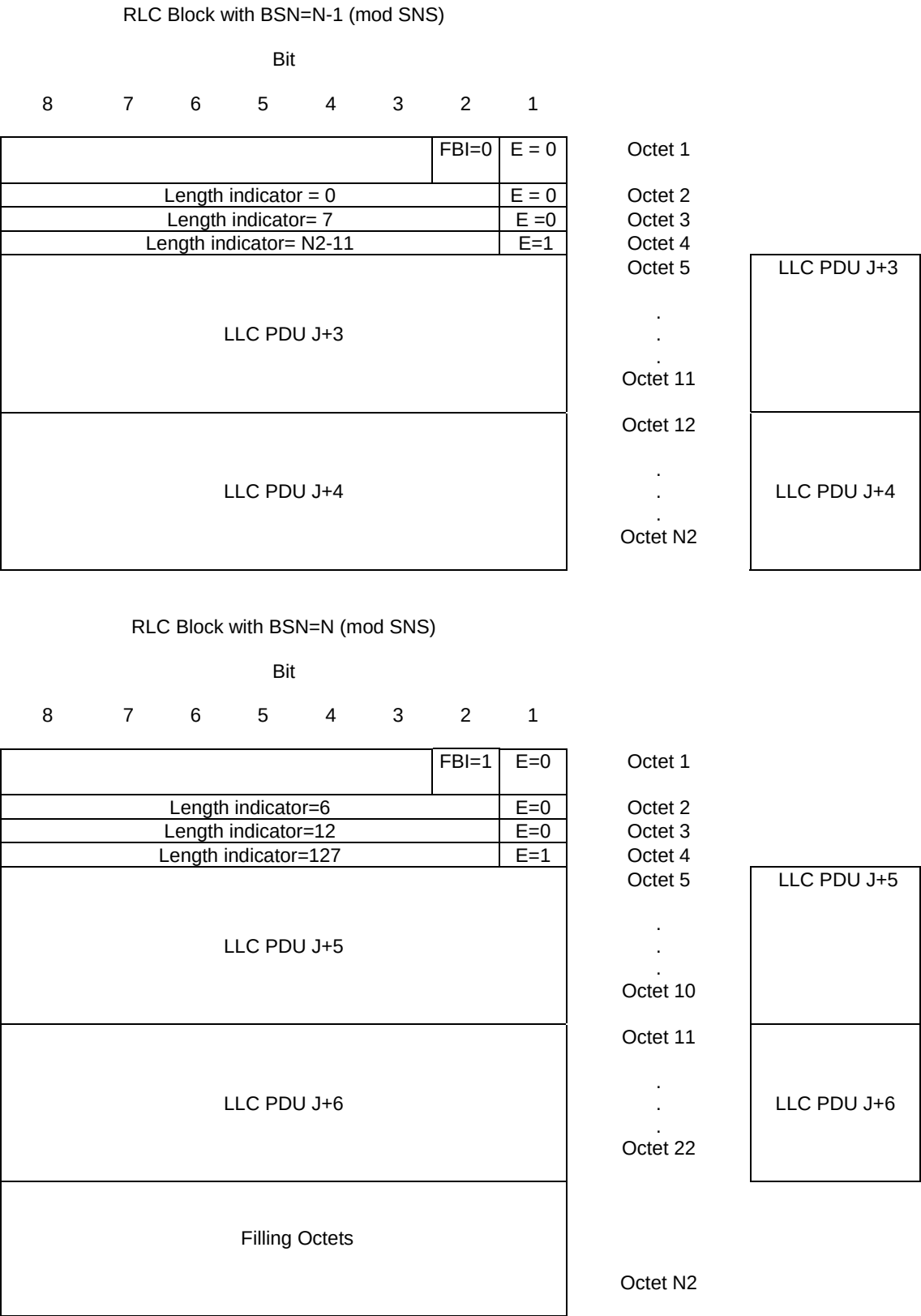
Figure B.9: Example for the case when the LLC PDU fills exactly the RLC data block (LLC PDU J+2 and LLC PDU J+4) and when the last LLC PDU cannot not fill the last RLC data block(LLC PDU J+6)
