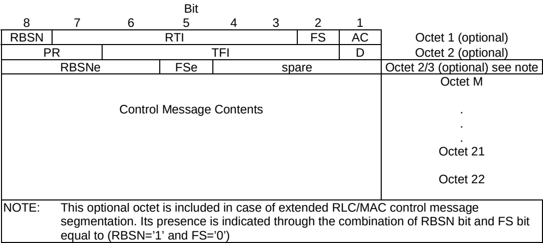
Figure 10.3.1.2.1: Downlink RLC/MAC control block message contents
