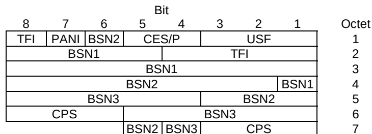
Figure 10.3a.3.5.2: DLMC Combined downlink RLC data block header for DAS-11 and DAS-12.
