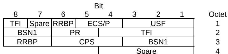
Figure 10.3a.3.2.5: EC-GSM-IoT downlink RLC data block header for MCS-5 and MCS-6
