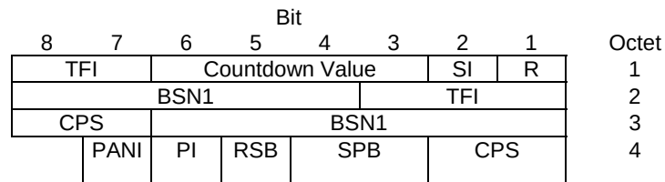
Figure 10.3a.4.3.2: EGPRS (FANR activated)/EGPRS2 uplink RLC data block header for MCS-1, MCS-2, MCS-3 and MCS-4
