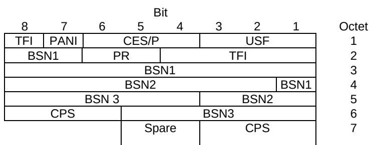
Figure 10.3a.3.8.1: Combined downlink RLC data block header for DBS-9 and DBS-10.
