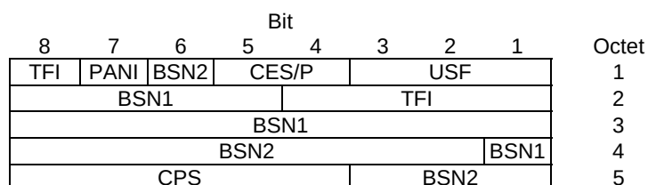
Figure 10.3a.3.1.4: DLMC EGPRS (FANR activated) / DLMC EGPRS2 downlink RLC data block header for MCS-7, MCS-8 and MCS-9
