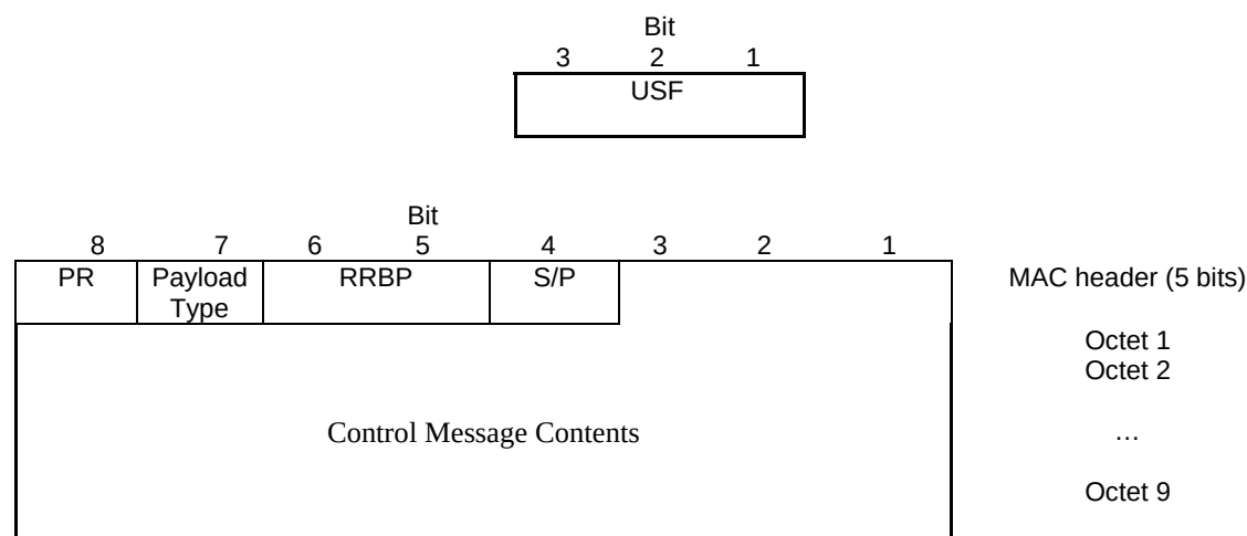
Figure 10.3.1.3.1: EC-GSM-IoT Downlink RLC/MAC control block together with its normal MAC header when Payload Type is set to 0
