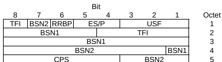
Figure 10.3a.3.1.3: DLMC EGPRS downlink RLC data block header (FANR not activated) for MCS-7, MCS-8 and MCS-9
