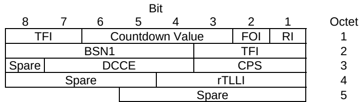
Figure 10.3a.4.2.3: EC-GSM-IoT uplink RLC data block header for MCS-5 and MCS-6
