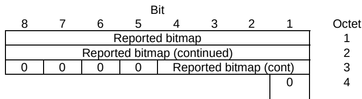
Figure 10.3a.6.1: Piggy-backed Ack/Nack field (Time-based)
