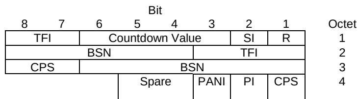
Figure 10.3a.4.6.1: Combined uplink RLC data block header for UBS-5, UBS-6.
