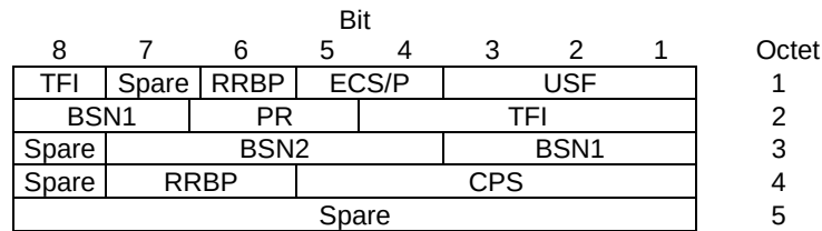
Figure 10.3a.3.1.5: EC-GSM-IoT downlink RLC data block header for MCS-7, MCS-8 and MCS-9
