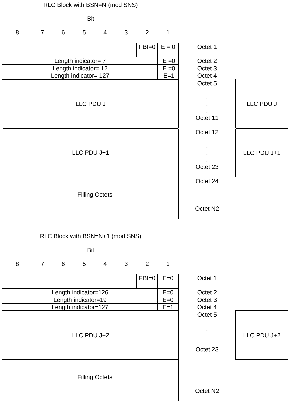
Figure B.11: Example for the case when the LLC PDU J+1 ends in the previous RLC data block and the start of the next LLC PDU J+2 is in the next RLC data block which is indicated using LI=126 as the first LI in that RLC data block.
