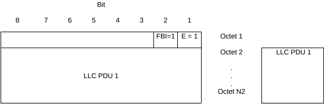
Figure B.10: Example for the case when a LLC PDU fills the RLC data block precisely.
