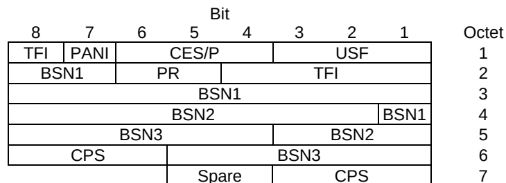
Figure 10.3a.3.5.1: Combined downlink RLC data block header for DAS-11 and DAS-12.
