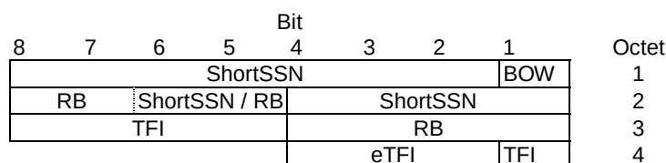
Figure 10.3a.5.2: Uplink Piggy-backed Ack/Nack field (SSN-based, eTFI assigned)
