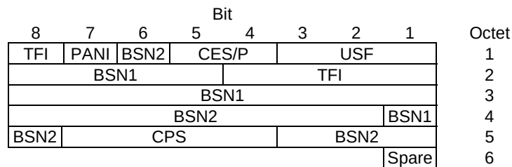
Figure 10.3a.3.4.2: DLMC Combined downlink RLC data block header for DAS-8 and DAS-9.
